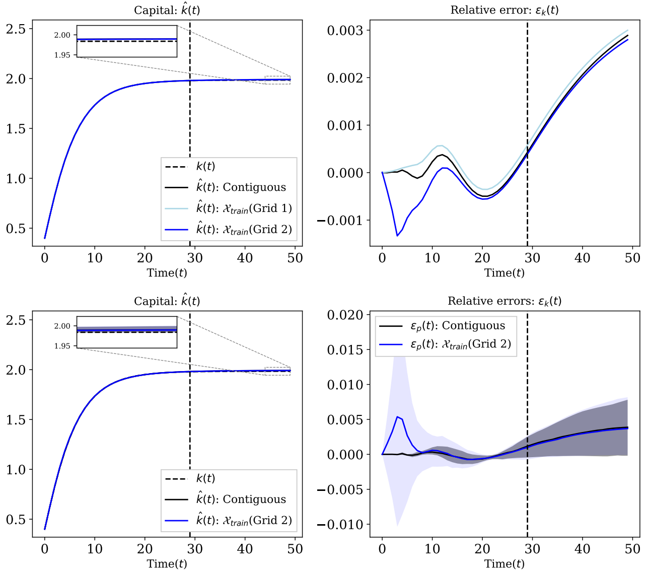
Figure 5: Comparison between the value function iteration and approximate solution using a deep neural network for the sequential neoclassical growth model. The first sparse grid is defined as \hat{X} (Grid 1) \equiv \{0, 1, 2, 4, 6, 8, 12, 16, 20, 24, 29\} and the second sparse grid is defined as \hat{X} (Grid 2) \equiv \{0, 1, 4, 8, 12, 16, 20, 24, 29\} . The top panels show the approximate capital paths and the relative errors between the approximate capital path and the capital path obtained by the value function iteration method, for \hat{X} (Grid 1), \hat{X} (Grid 2), and the contiguous grid. The bottom panels show the median of the approximate capital paths and the median of relative errors for \hat{X} (Grid 1), \hat{X} (Grid 2), and the contiguous grid. The shaded regions show the 10th and the 90th percentiles. The dashed curves, denoted by k(t) , show the capital and path obtained by the value function iteration method. The dashed vertical line separates the interpolation from the extrapolation region.
