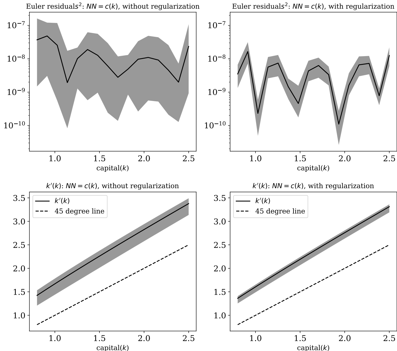
Figure 16: The effect of the L_2 explicit regularization on the solutions, when the consumption function c(k) is approximated with a deep neural network. The left panels show the results without regularization. The right panels show the results with L_2 regularization with penalization coefficient \lambda = 10^{-9} . The solid curves in the top panels show the median of the Euler residuals squared. The solid curves in the bottom panels show the median of the approximate policy functions for capital, i.e., k'(k; c(\cdot)) . The shaded regions show the 10th and the 90th percentiles.
